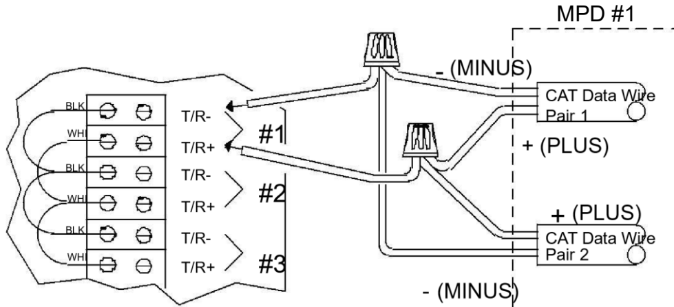
Fig. 9, How to Connect More than Eight, Dispenser Control Data wires
