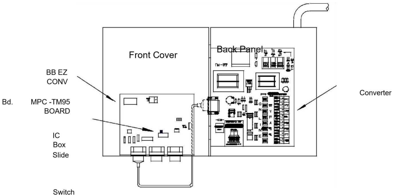
Fig. 4, The PetroSmart EZ Wayne Dispenser Control Box with the Door Open.
