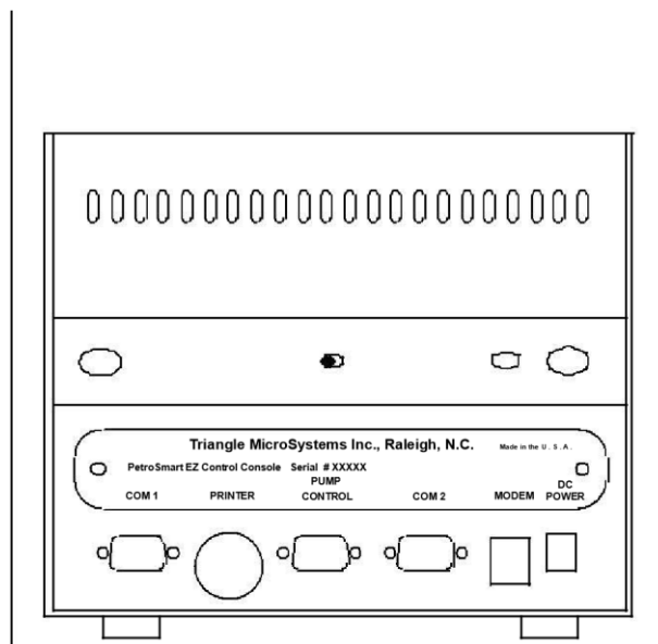
Fig. 12, Back View of the PetroSmart EZ Console
