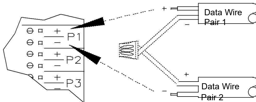
Fig. 6, How to Connect More than Eight, Dispenser Control Data wires
