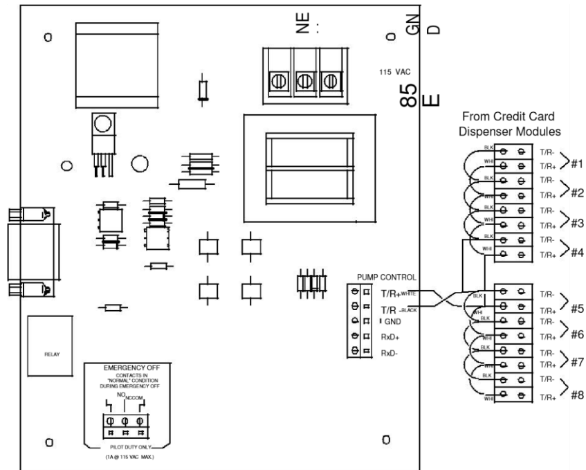
Fig. 8, PetroSmart Cat Interface MPC-TM84E Board
