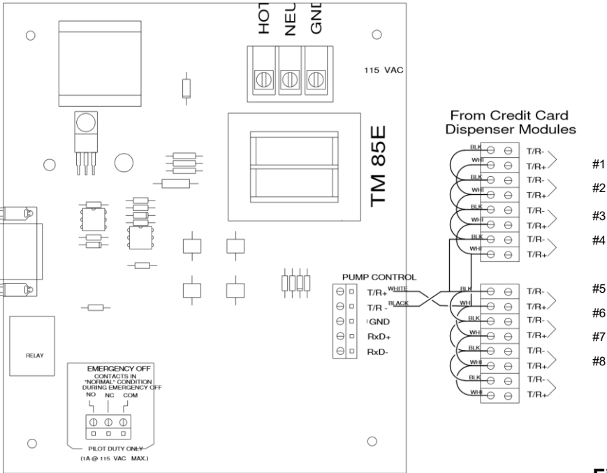
PetroSmart DPT Interface MPC-TM85 Board
