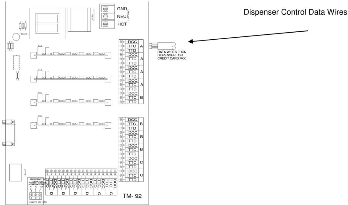
Fig. 5, Dispenser Control MPC-TM92 Board
