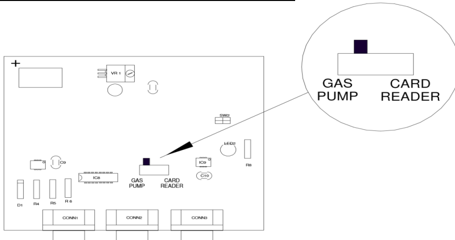
Fig. 9, PETROSMART EZ Converter Board
