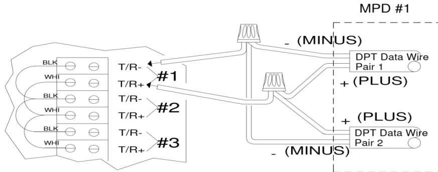
Fig. 8, How to Connect More than Eight, Dispenser Control Data wires
